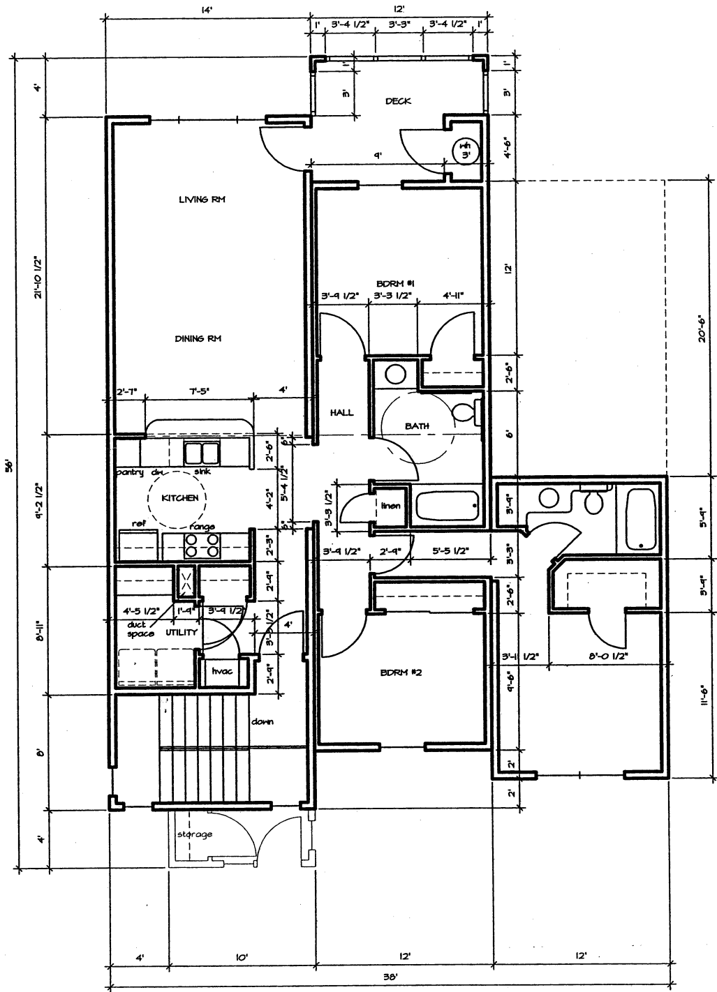
2ND FLOOR 3-BDRM FLAT UNIT 1/4"=1'-0" 1199 sq ft excluding common mudroom
